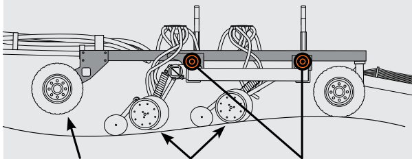
Tire Leaves Ground Poor Seed Depth Control Rigidly Mounted to Frame
